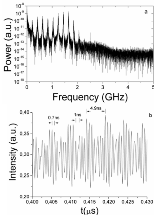
Fig. 5. (a) Power spectra corresponding for feedback ratio ( \gamma=10\% ), I=1.04 \cdot I_{0\text{th}} , T=24^\circ\text{C} , and L=70\text{cm} , in the LFF regime; (b) Zoom on intensity time series; two time scale are evident 4.9\text{ns} ( \nu_{\text{EC}}=204\text{MHz} ) corresponding to the period of the external cavity modes and 0.7\text{ns} ( \nu_{\text{SC}} \approx 1.43\text{GHz} ) corresponding to the duration of the fast pulsation from the short external cavity.
