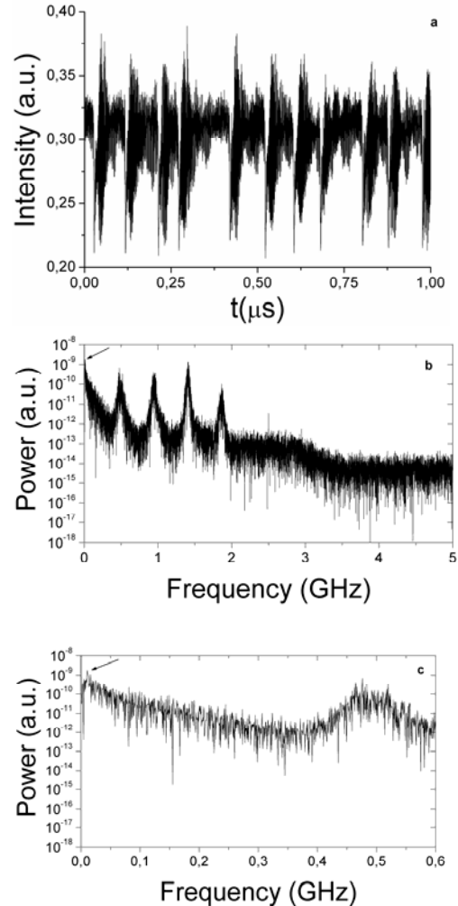
Fig. 2. Laser emission at LFF regime. a) intensity time series of a SL subject to constant feedback ratio, \gamma=10\% , I=1.04 \cdot I_{\text{th}} , T=24^\circ\text{C} , L=31.5 cm; (b) the power spectra corresponding to 2 (a); (c) zoom-in of 2 (b); the arrows point to the LFF frequency of 12.1 MHz.
